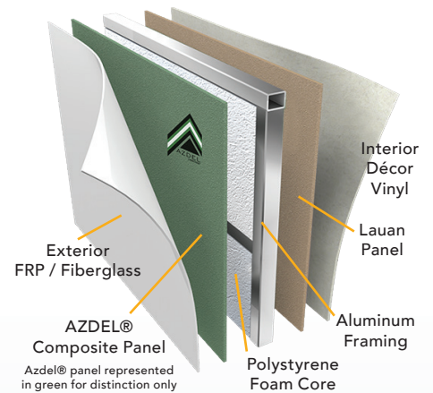
E-SERIES SIDEWALL CUT-AWAY LAMINATED AZDEL ONBOARD® COMPOSITE WALLS WITH ALUMINUM FRAMING AND GEL-COATED FIBERGLASS
